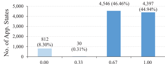
(c) Analysis Result of GPSLogger-new (Extended)
